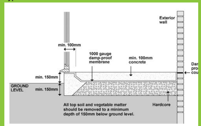
Typical solid floor detail
